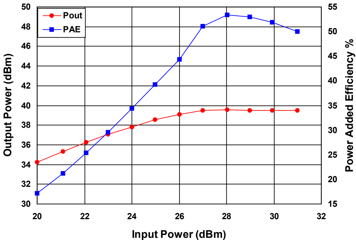
TGF4118 RF Performance at F = 2.3 GHz V_d = 8.0\text{ V} , V_g = -1.1\text{ V} , I_q = 1.69\text{ A} and T_A = 25^\circ\text{C}
