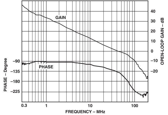
TPC 49. Open-Loop Frequency Response
