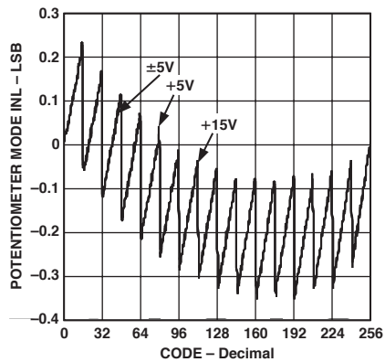
TPC 5. INL vs. Code vs. Supply Voltages
