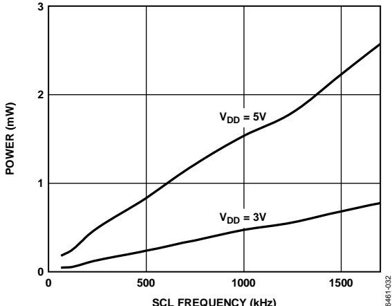
Figure 17. Power vs. SCL Frequency, V REF = 2.5 V
