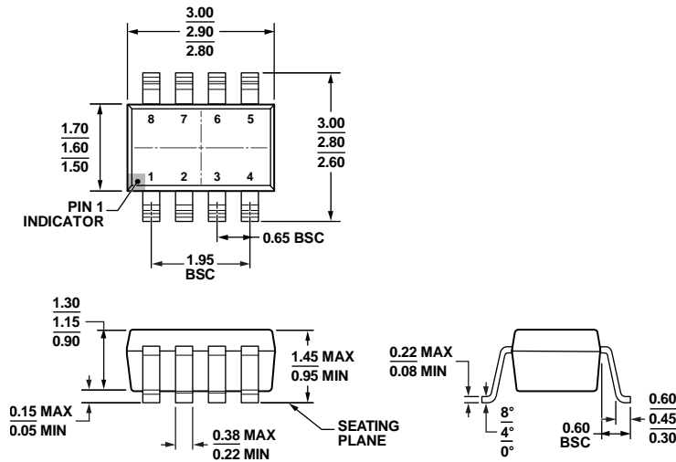
COMPLIANT TO JEDEC STANDARDS MO-178-BA Figure 29. 8-Lead Small Outline Transistor Package [SOT-23] (RJ-8) Dimensions shown in millimeters
