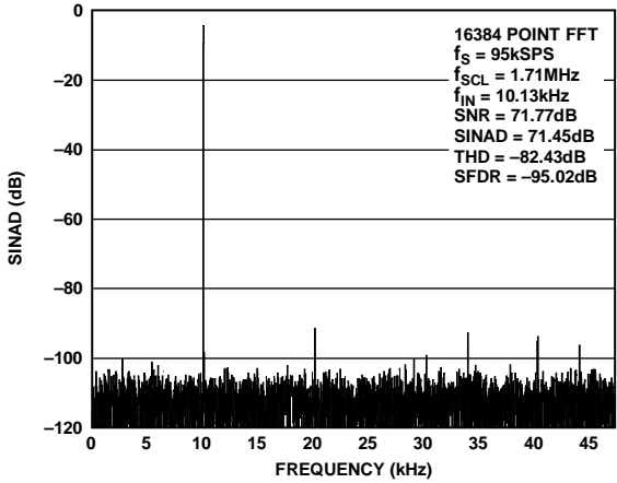
Figure 16. Dynamic Performance, f SCL = 1.71 MHz Without Clock Stretching, V DD = 5 V, Full-Scale Input, Seven-Term Blackman-Harris Window
