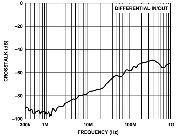
Figure 28. AD8117 Crosstalk, One Adjacent Channel
