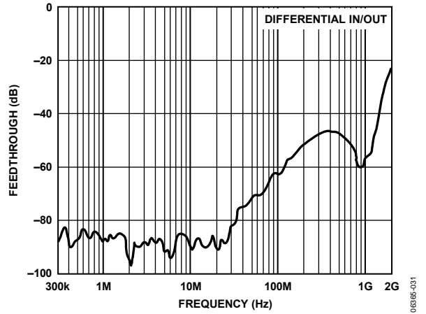
Figure 36. AD8117 Crosstalk, Off Isolation
