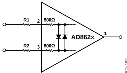
Figure 54. Input Protection
