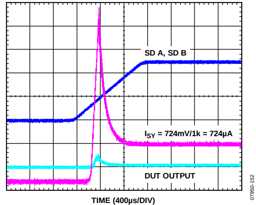
Figure 59. Shutdown Pin Rise Time = 1 ms
