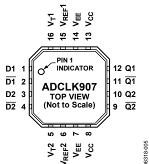
Figure 5. ADCLK907 Pin Configuration
