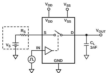
Figure 28. Charge Injection
