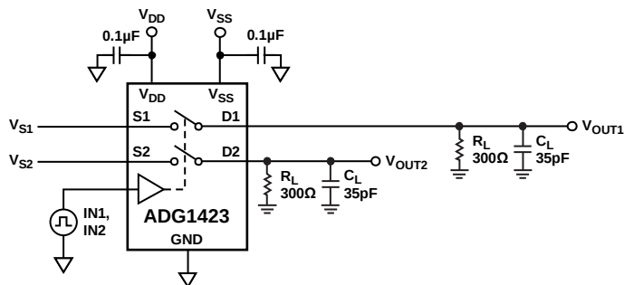
Figure 27. Break-Before-Make Time Delay
