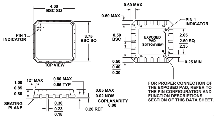
Figure 40. 20-Lead Lead Frame Chip Scale Package [LFCSP_VQ] 4 mm × 4 mm Body, Very Thin Quad (CP-20-4)
