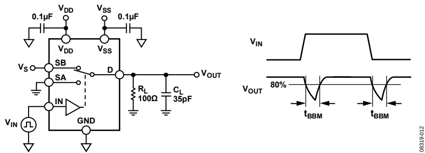
Figure 30. Break-Before-Make Delay, t_D
