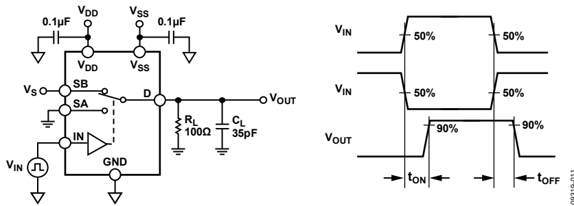
Figure 29. Switching Timing
