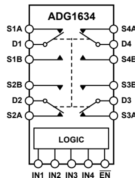
Figure 3. ADG1634 LFCSP_VQ
