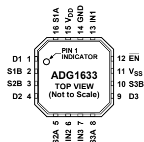
Figure 5. ADG1633 LFCSP_VQ Pin Configuration
