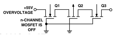
Figure 5. +55 V Overvoltage with Power OFF
