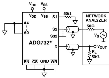
Test Circuit 11. Channel-to-Channel Crosstalk
