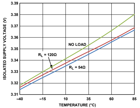
Figure 26. ADM2687E Isolated Supply Voltage vs. Temperature ( V_{CC} = 5\text{ V} , Data Rate = 500 kbps)
