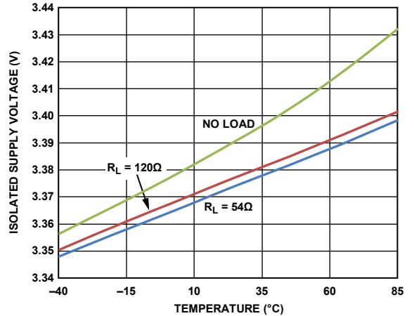
Figure 24. ADM2682E Isolated Supply Voltage vs. Temperature ( V_{CC} = 5\text{ V} , Data Rate = 16 Mbps)
