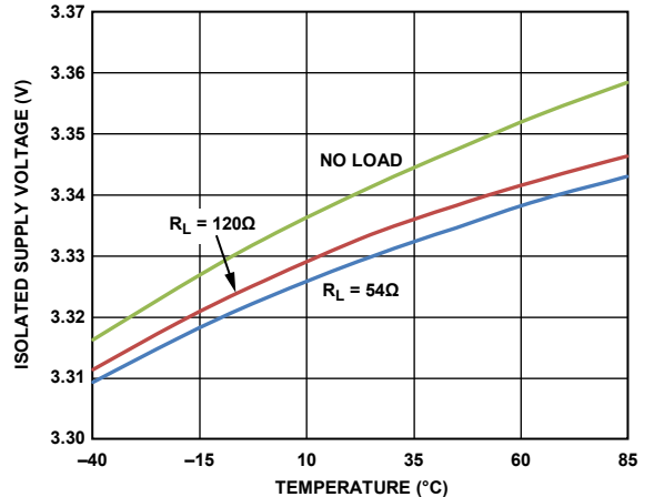
Figure 25. ADM2687E Isolated Supply Voltage vs. Temperature ( V_{CC} = 3.3\text{ V} , Data Rate = 500 kbps)
