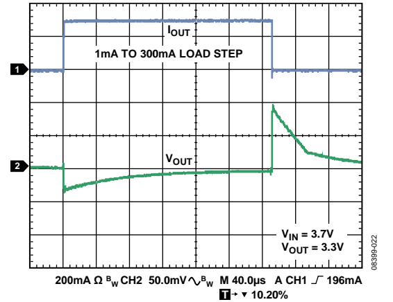
Figure 26. Load Transient Response, C_{OUT} = 1\text{ }\mu\text{F}
