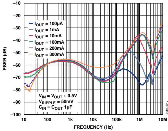
Figure 21. Power Supply Rejection Ratio vs. Frequency, V_{OUT} = 4.2\text{ V} , V_{IN} = 4.7\text{ V}
