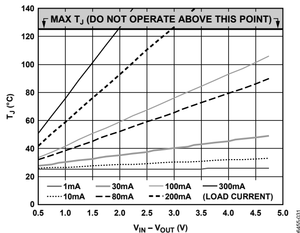
Figure 35. 0 mm 2 of PCB Copper, T_A = 25^\circ\text{C}
