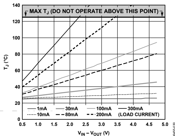
Figure 34. 100 mm 2 of PCB Copper, T_A = 25^\circ\text{C}
