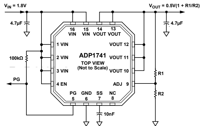
Figure 2. ADP1741 with Adjustable Output Voltage, 0.75 V to 3.0 V
