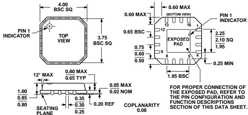
Figure 49. 16-Lead Lead Frame Chip Scale Package [LFCSQ_VQ] 4 mm × 4 mm Body, Very Thin Quad (CP-16-4) Dimensions shown in millimeters
