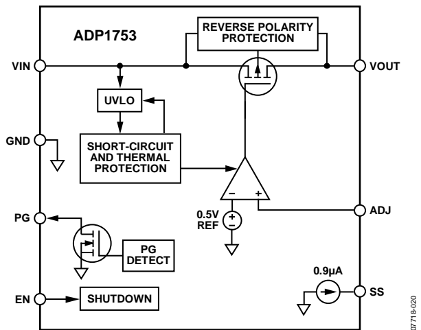
Figure 25. ADP1753 Internal Block Diagram
