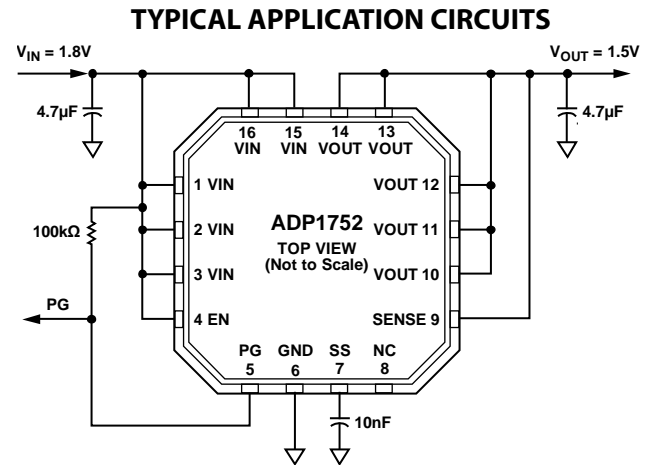
Figure 1. ADP1752 with Fixed Output Voltage, 1.5 V
