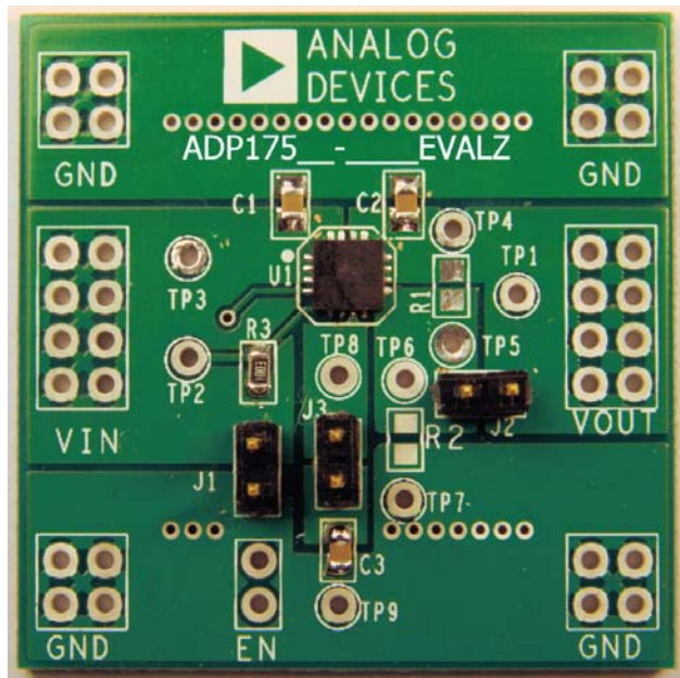
Figure 46. Evaluation Board
