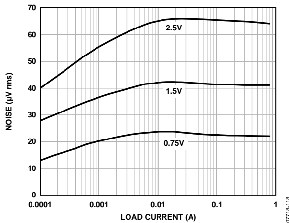
Figure 18. Noise vs. Load Current and Output Voltage
