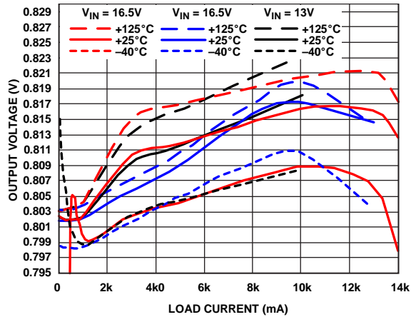
Figure 16. Output Voltage Accuracy—600 kHz, V_{OUT} = 0.8\text{ V}
