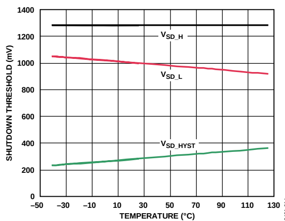
Figure 15. Shutdown Threshold vs. Temperature
