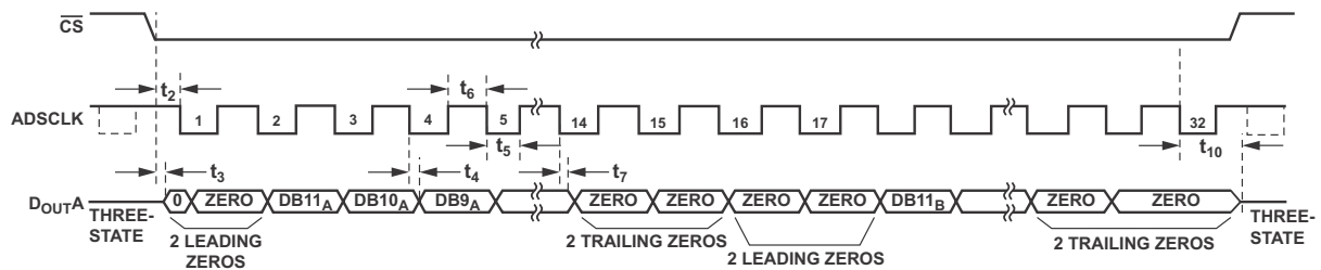
Figure 88. Reading Data from Both ADCs on One D_{\text{OUT}} Line with 32 ADSClks
