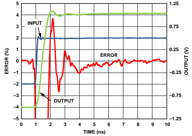
Figure 31. ADV3220 Settling Time 2 V Output Step
