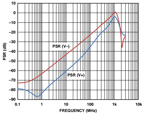
Figure 29. ADV3219 PSR
