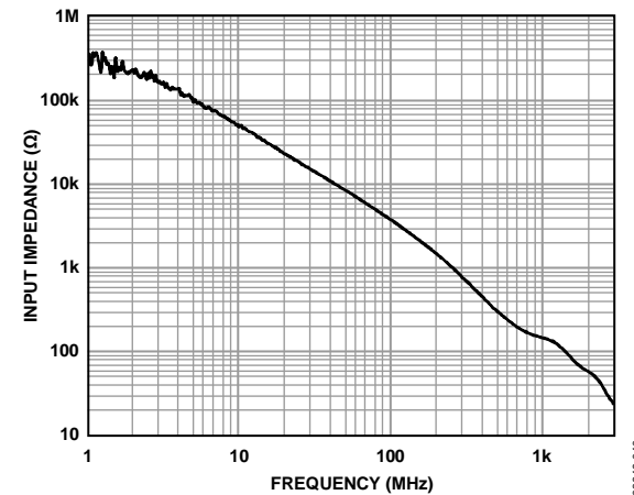
Figure 39. ADV3219/ADV3220 Input Impedance vs. Frequency
