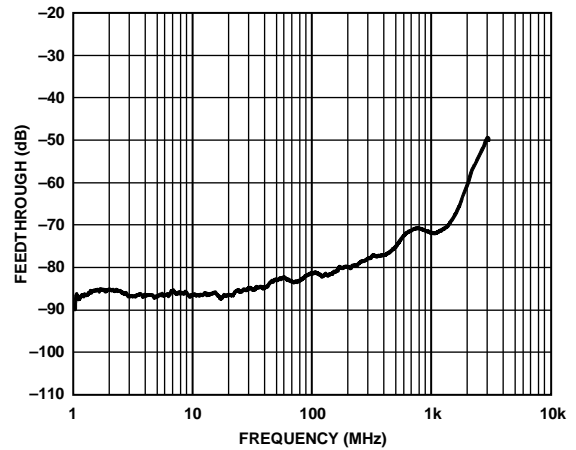
Figure 38. ADV3220 Off Isolation vs. Frequency
