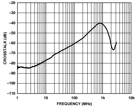
Figure 37. ADV3220 Crosstalk vs. Frequency
