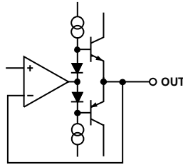
Figure 51. ADV3219 Enabled Analog Output
