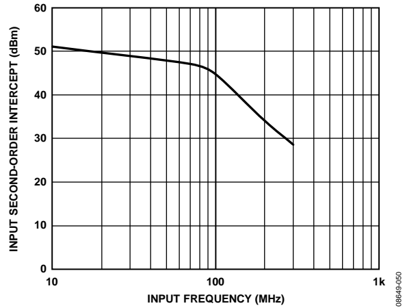
Figure 48. ADV3220 Input Second-Order Intercept, R_L = 100 \Omega , C_L = 4 \text{ pF} , 0 dBm Input
