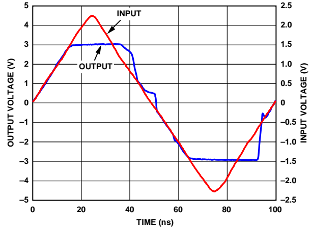
图51. ADV3222过驱恢复时
