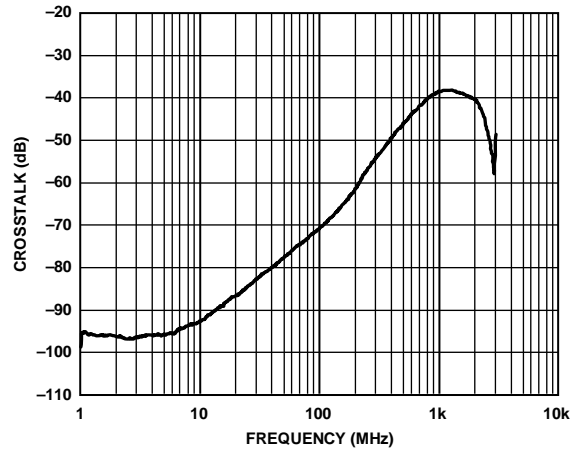
图40. ADV3222邻道串扰
