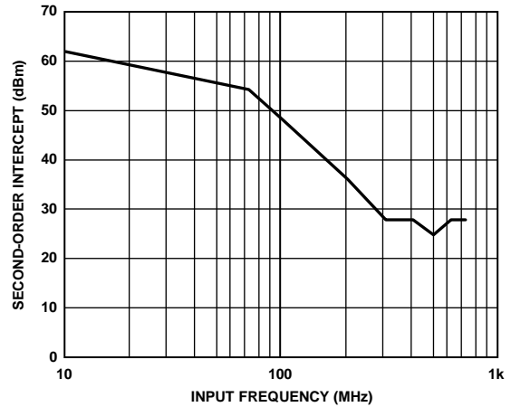
图52. ADV3222输入二阶交调点 ( R_L = 100 \Omega , C_L = 4 \text{ pF} )
