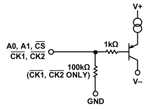
图58. ADV3221/ADV3222逻辑输入
