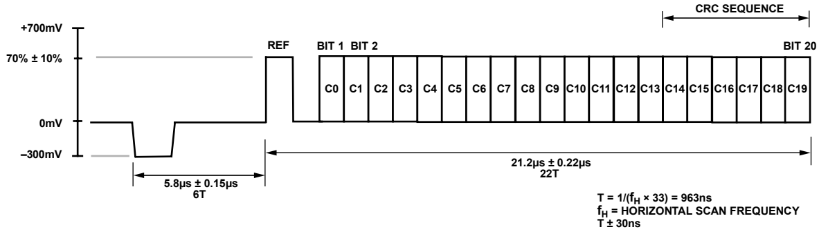
Figure 92. Enhanced Definition (525p) CGMS Waveform
