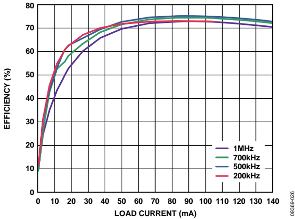
Figure 15. 5 V In to 15 V Out Efficiency at Various Switching Frequencies with Halo Transformer
