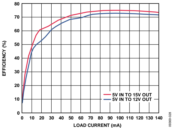
Figure 17. Double-Supply Efficiency with Coilcraft Transformer at 500 kHz f_{SW}
