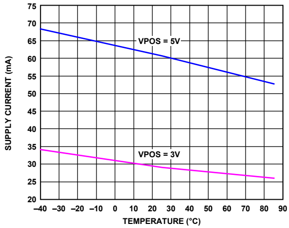
Figure 51. Supply Current vs. Temperature, 3 V and 5 V
