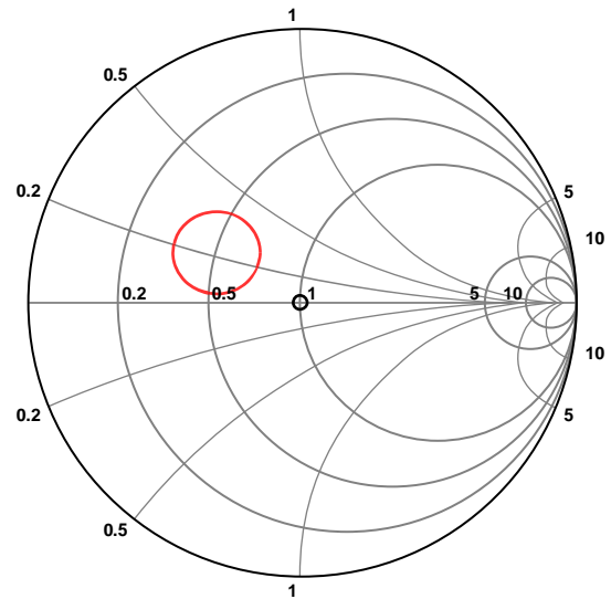
Figure 61. Area of Optimal Noise Matching for ADL5523
