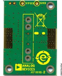
Figure 56. Evaluation Board Layout (Bottom View)
