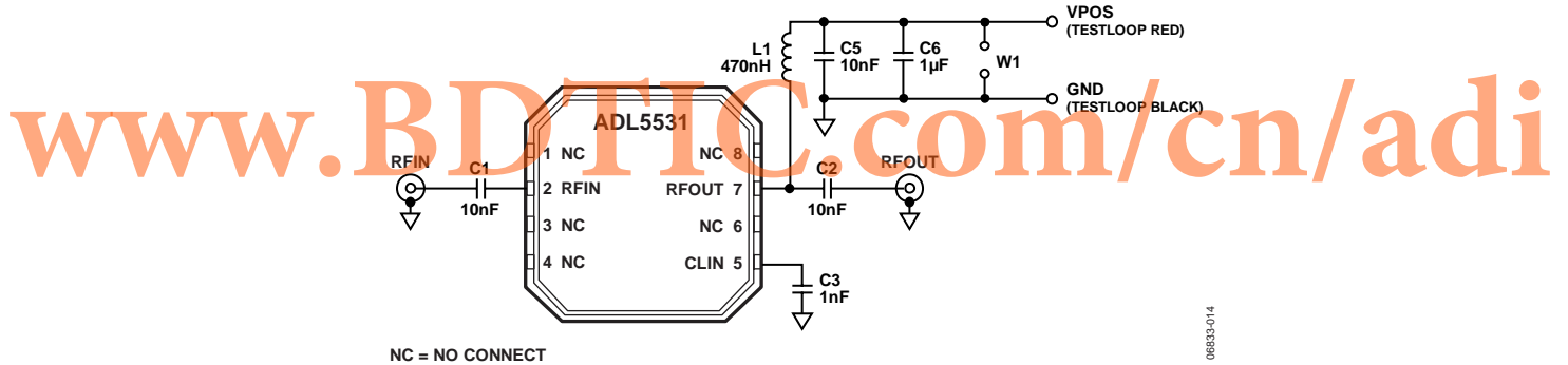
Figure 16. Basic Connections
