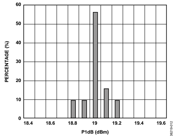
Figure 11. P1dB Distribution at 900 MHz
