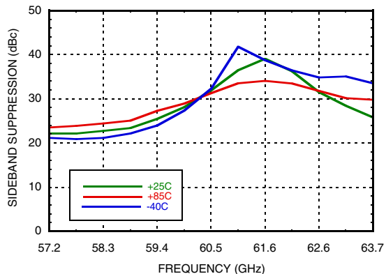
Figure 23. Sideband Suppression vs. Frequency over Temperature [2]
