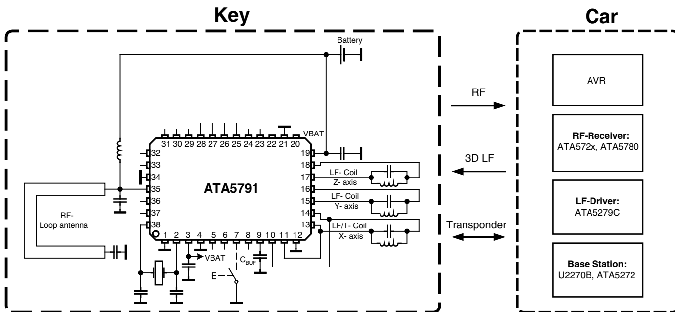
Figure 1-1. System Block Diagram
