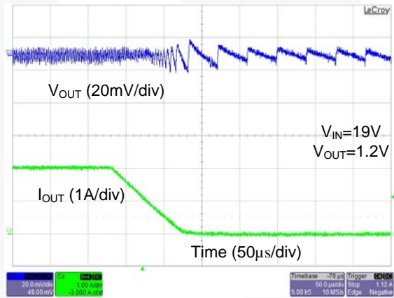
Figure 21. Operation as Load Changes from 2 A to 0 A
