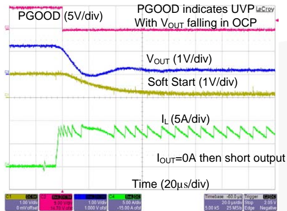
Figure 24. Over-Current Protection with Heavy Load Applied
