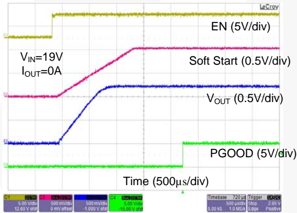
Figure 14. Startup Waveforms with 0 A Load Current
