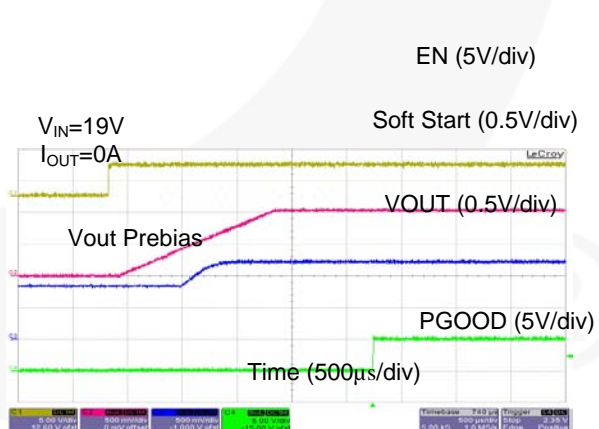
Figure 17. Startup Waveforms with Pre-bias Voltage on Output
