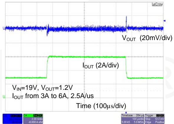
Figure 23. Load Transient from 50% to 100% Load Current
