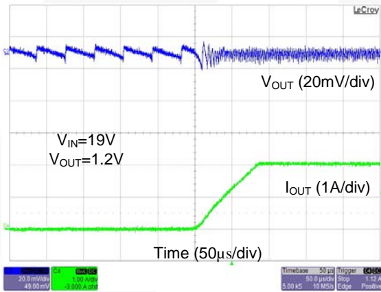
Figure 20. Operation as Load Changes from 0 A to 2 A
