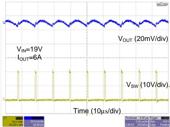
Figure 19. Static Load Ripple at Full Load
