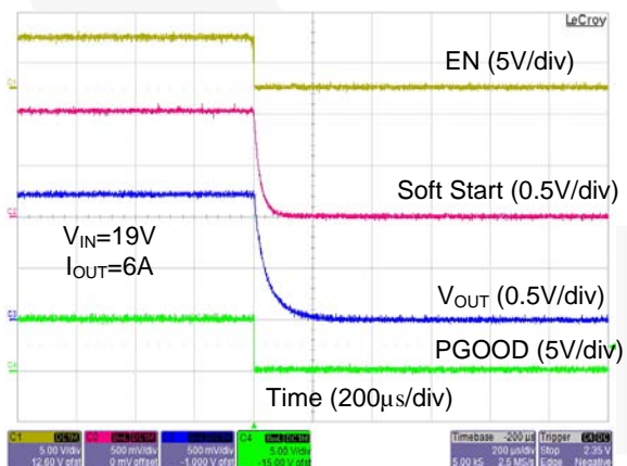
Figure 16. Shutdown Waveforms with 10 A Load Current
