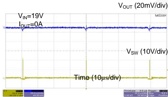
Figure 18. Static Load Ripple at Light Load
