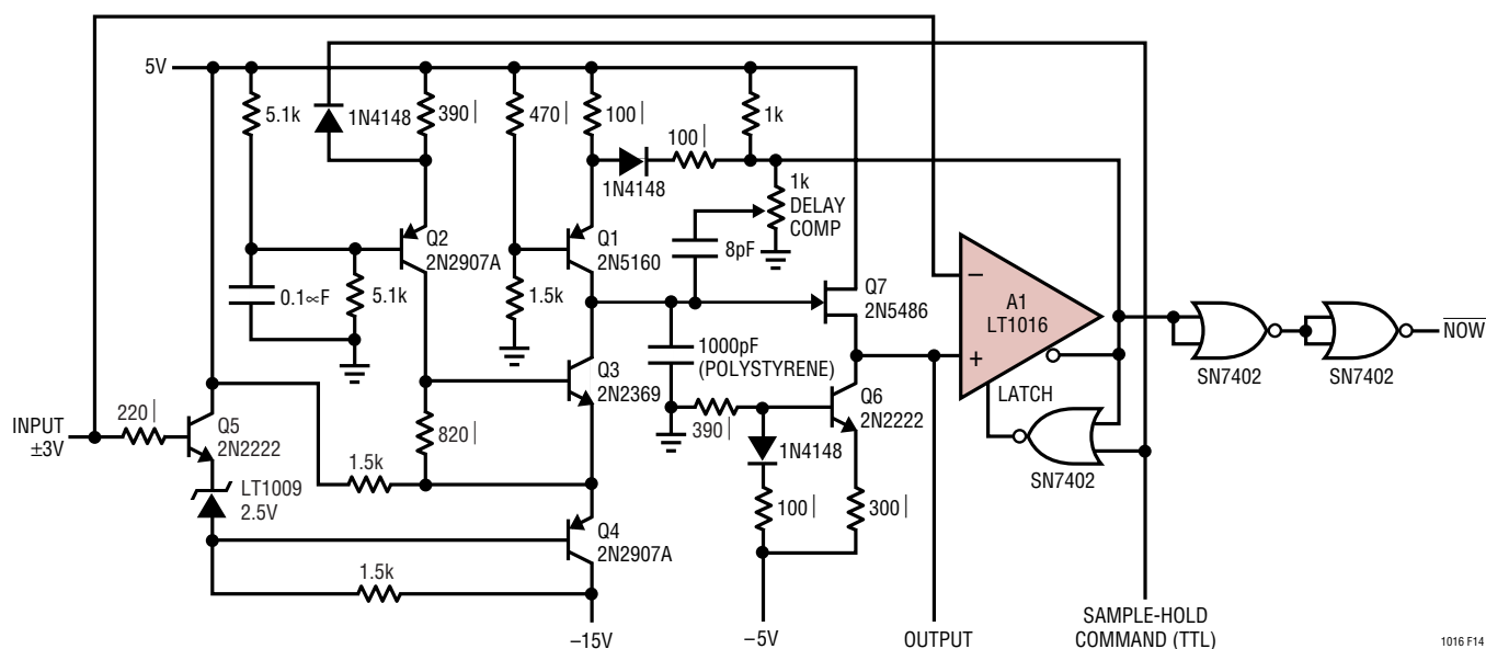
Figure 14. 200ns Sample-and-Hold
