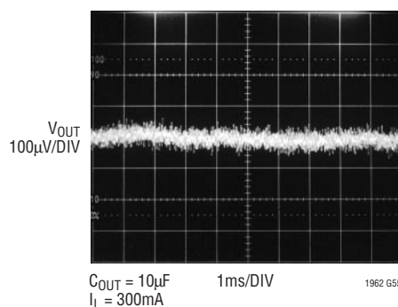
LT1962-5 10Hz to 100kHz Output Noise ( C_{BYP} = 0.01μF )
