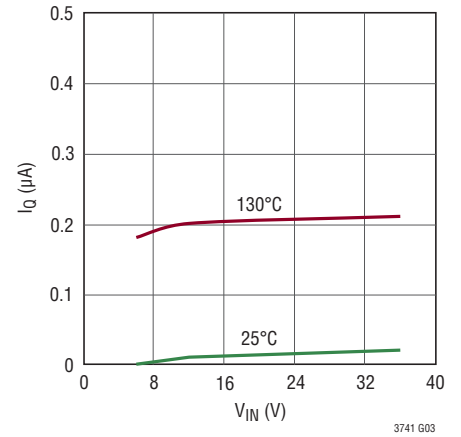
I Q in Shutdown
