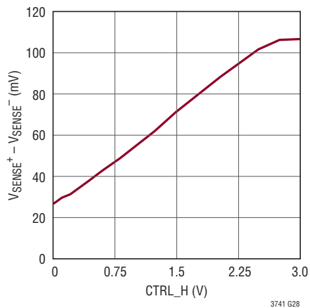
Overcurrent Threshold
