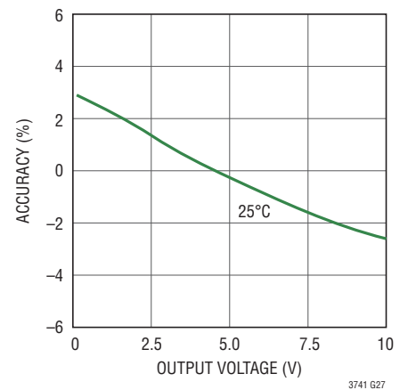
Current Regulation Accuracy CTRL1 = 0.75V, V_{IN} = 12V
