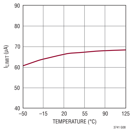
RT Pin Current Limit
