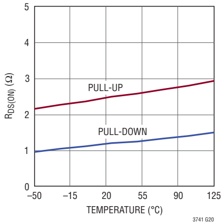
HG Driver R_{DS(ON)}
