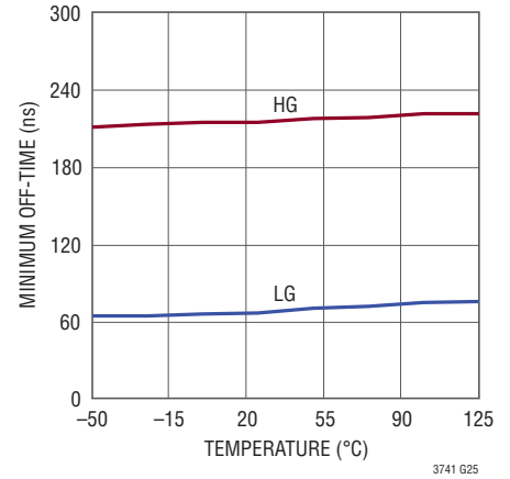
Minimum Off-Time
