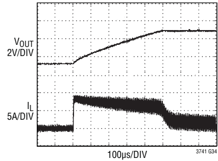
Voltage Regulation with 10A Regulated Inductor Current
