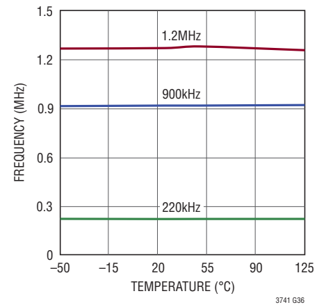
Oscillator Frequency
