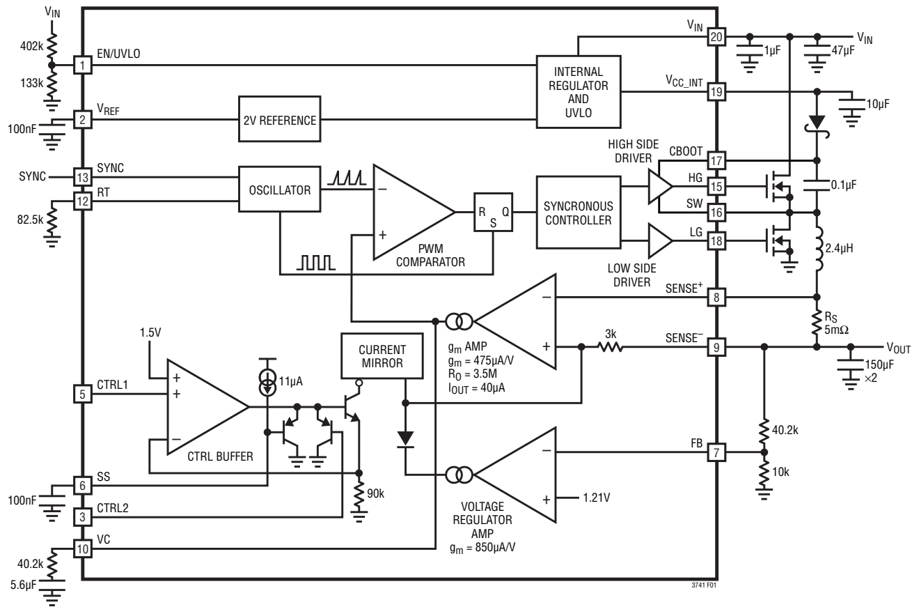
Figure 1. Block Diagram
