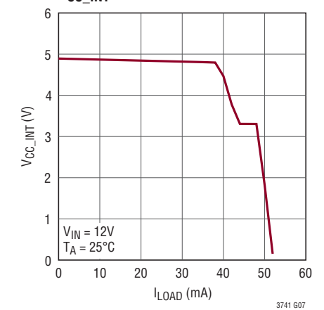
V CC_INT Current Limit
