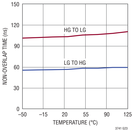
Non-Overlap Time
