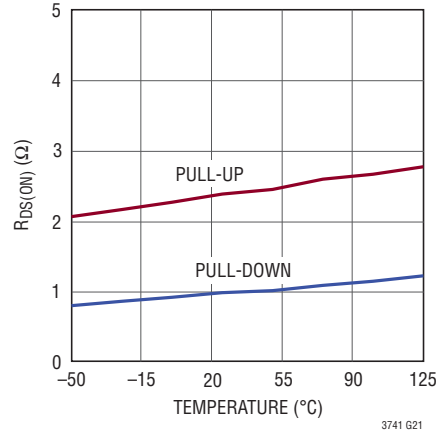
LG Driver R_{DS(ON)}
