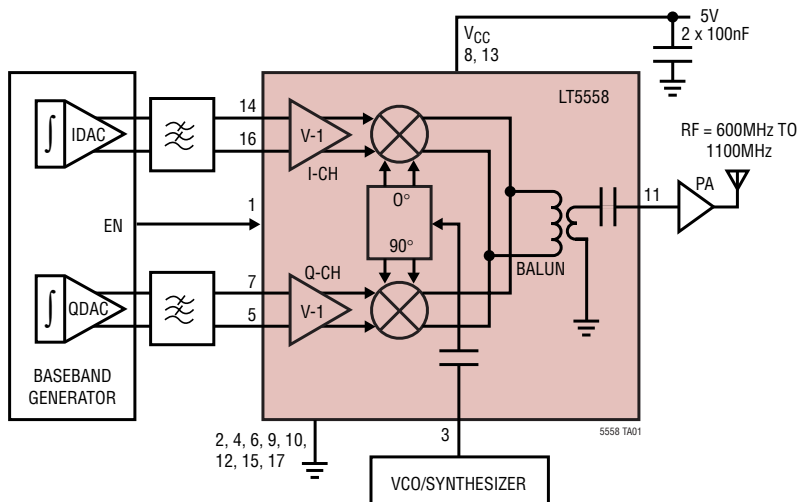
600MHz to 1100MHz Direct Conversion Transmitter Application
