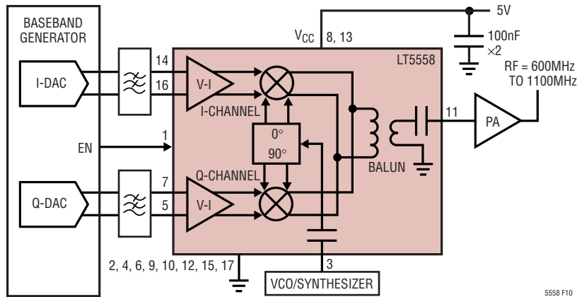
Figure 10. 600MHz to 1.1GHz Direct Conversion Transmitter Application
