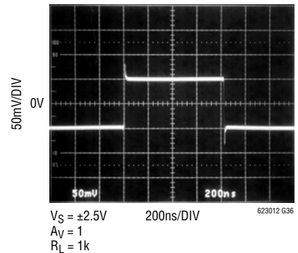
Small-Signal Response
