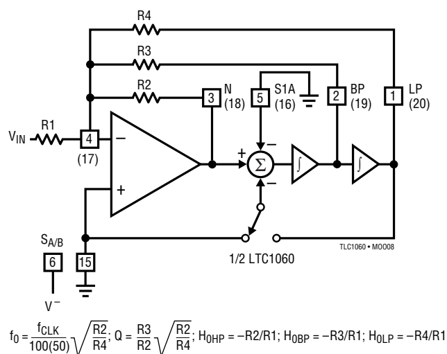
Figure 11. Mode 3: 2nd Order Filter Providing Highpass, Bandpass, Lowpass
