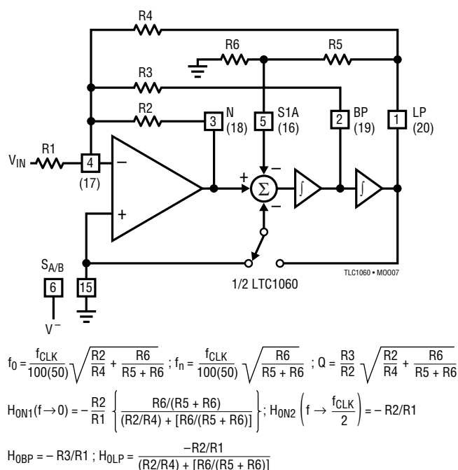
Figure 10. Mode 2b: 2nd Order Filter Providing Notch, Bandpass, Lowpass
