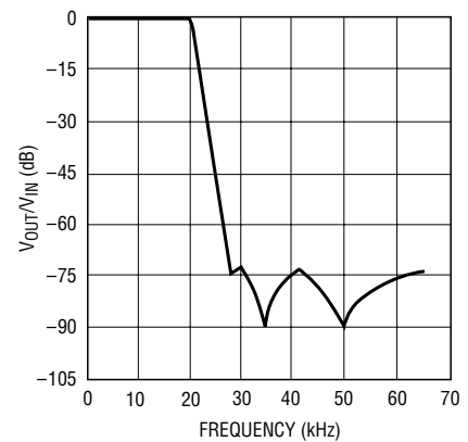
Amplitude Response
