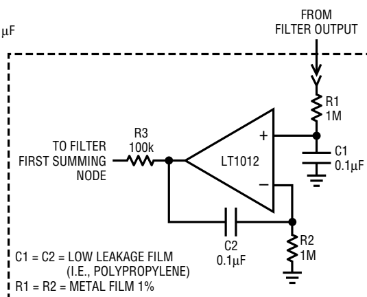
Figure 4. Servo Amplifier
