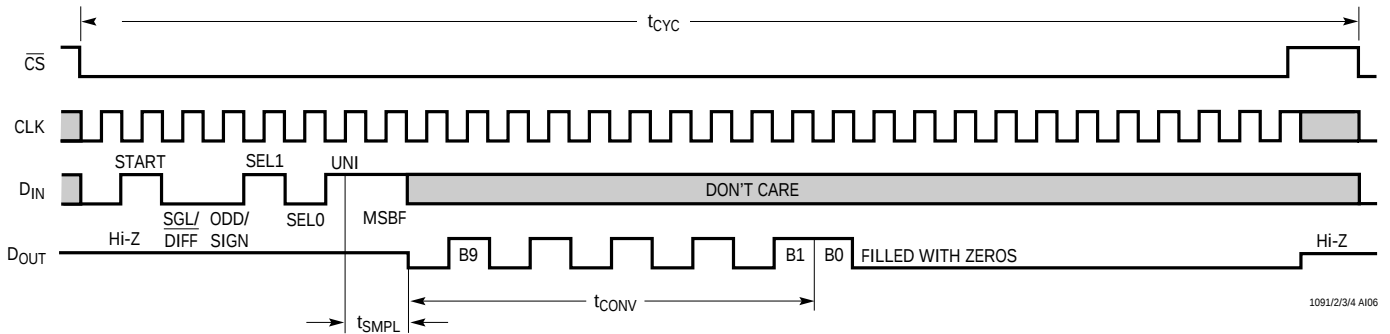
LTC1093/LTC1094 Operating Sequence Example: Differential Inputs (CH4 + , CH5 - ), Unipolar Mode
