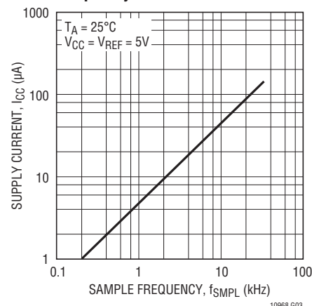
Supply Current vs Sample Frequency LTC1096
