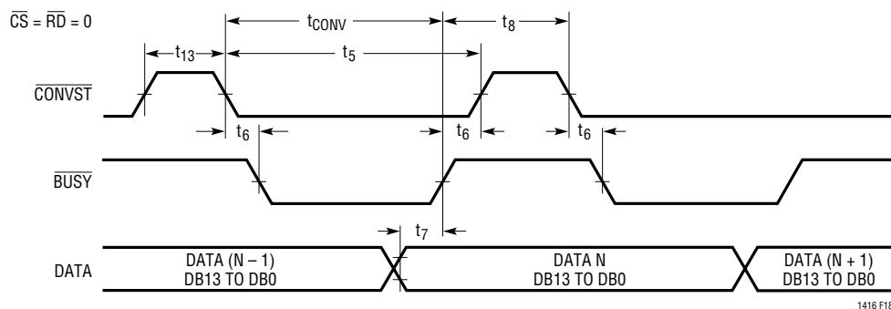
Figure 18. Mode 1b. \overline{CONVST} Starts a Conversion. Data Outputs Always Enabled ( \overline{CONVST} = \text{[Pulse]} \text{ )}
