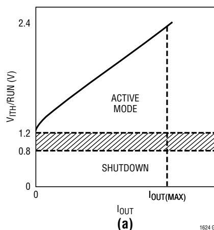
V_{ITH} vs Output Current
