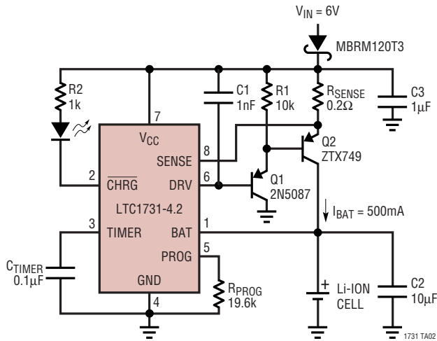
Linear Charger Using a PNP Transistor
