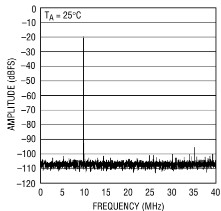
Averaged 8192 Point FFT, 70.2MHz Input, -20dB, 3.2V Range
