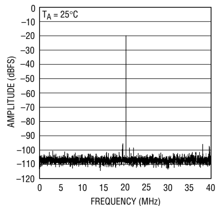
Averaged 8192 Point FFT, 20.2MHz Input, -20dB, 3.2V Range
