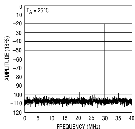
Averaged 8192 Point FFT, 50.2MHz Input, -20dB, 3.2V Range
