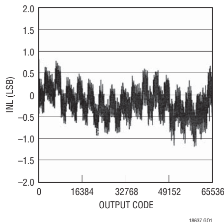
Integral Nonlinearity vs Output Code (LTC1867)
