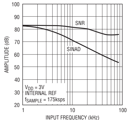
Signal-to-(Noise + Distortion) Ratio vs Input Frequency
