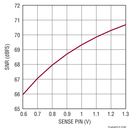
LTC2144-12: SNR vs SENSE, f_{IN} = 5\text{MHz} , -1dBFS
