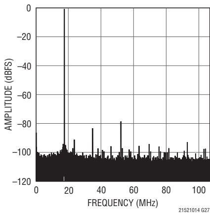
LTC2151-14: 32K Point FFT, f_{IN} = 227\text{MHz} , -1dBFS, 210Msps
