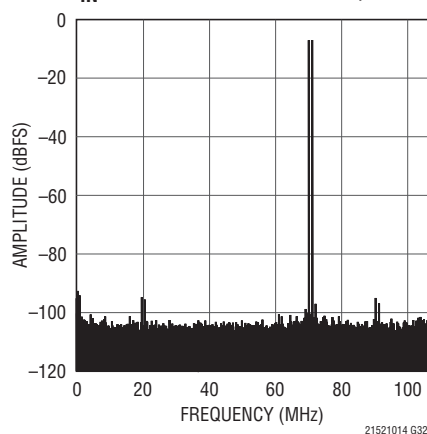
LTC2151-14: 32K Point 2-Tone FFT, f_{IN} = 70.5\text{MHz} and 69.5\text{MHz} , 210Mps
