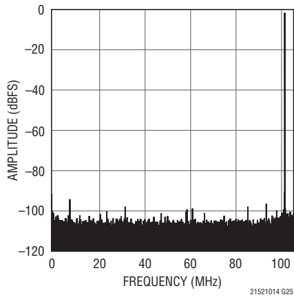
LTC2151-14: 32K Point FFT, f_{IN} = 101\text{MHz} , -1dBFS, 210Msps
