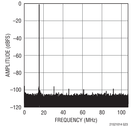
LTC2151-14: 32K Point FFT, f_{IN} = 15\text{MHz} , -1dBFS, 210Msps
