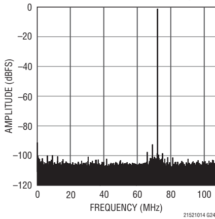
LTC2151-14: 32K Point FFT, f_{IN} = 71\text{MHz} , -1dBFS, 210Msps
