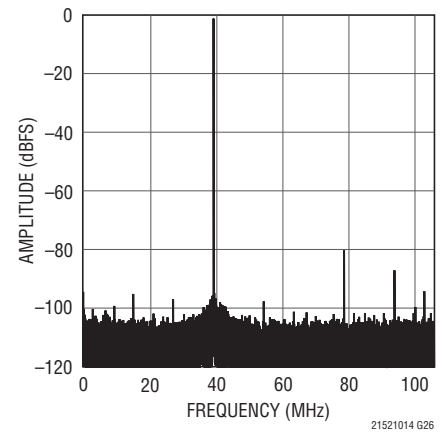
LTC2151-14: 32K Point FFT, f_{IN} = 171\text{MHz} , -1dBFS, 210Msps
