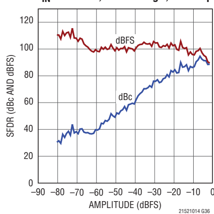
LTC2151-14: SFDR vs Input Level, f_{IN} = 71\text{MHz} , 1.5V Range, 210Mps
