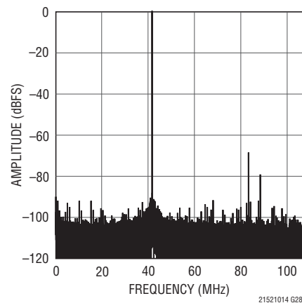
LTC2151-14: 32K Point FFT, f_{IN} = 379\text{MHz} , -1dBFS, 210Msps
