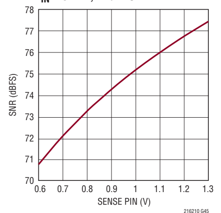
LTC2160: SNR vs SENSE, f_{IN} = 5\text{MHz} , -1\text{dBFS}
