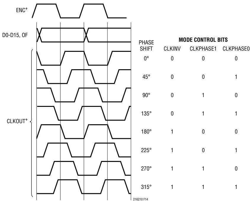
Figure 14. Phase-Shifting CLKOUT
