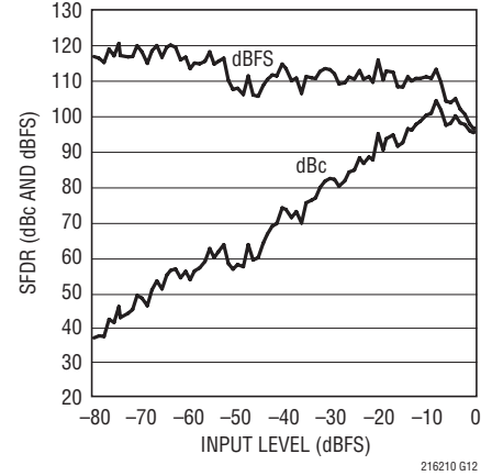
LTC2162: SFDR vs Input Level, f_{IN} = 70\text{MHz} , 65Mpsps, 2V Range
