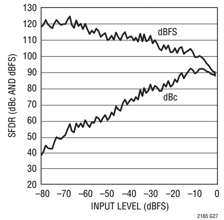
LTC2163 SFDR vs Input Level, f_{IN} = 70\text{MHz} , 2\text{V} Range, 80Mps
