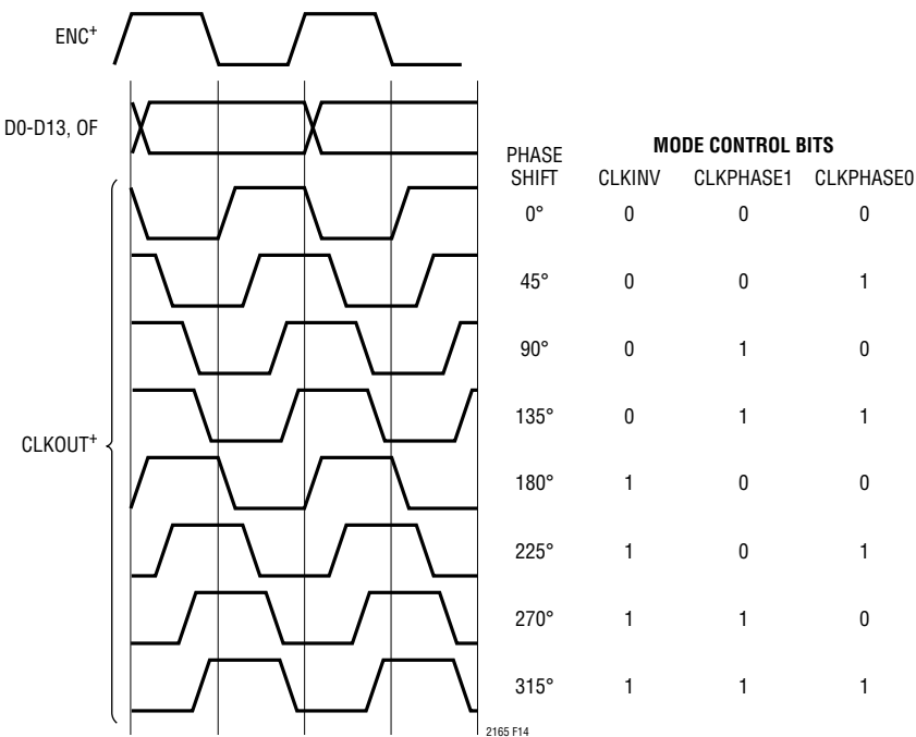
Figure 14. Phase-Shifting CLKOUT
