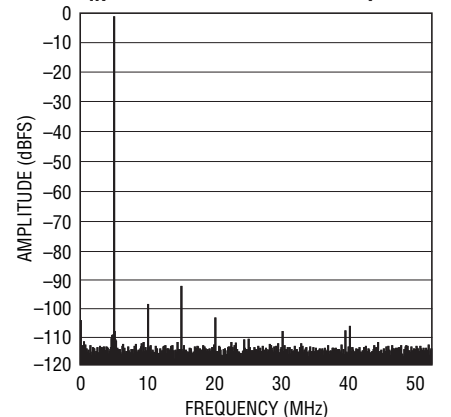
LTC2164 64k Point FFT, f_{IN} = 5\text{MHz} , -1dBFS, 105Mps
