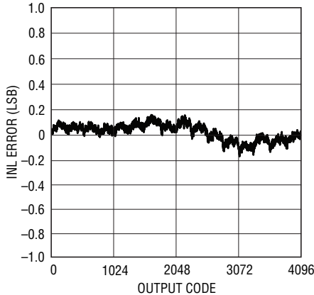
LTC2172-12: Integral Nonlinearity (INL)
